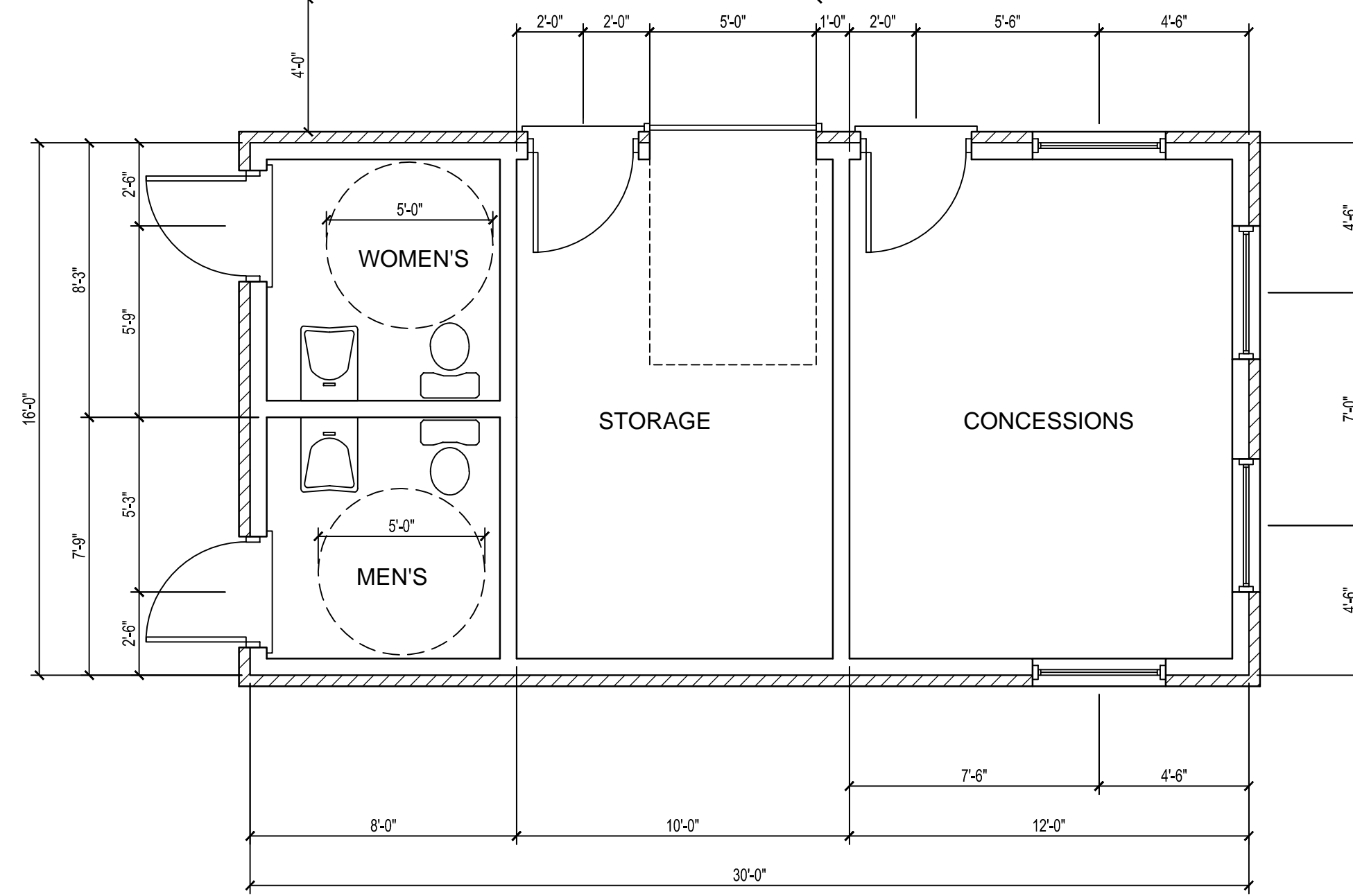
FIRST FLOOR PLAN SCALE: 1/4"=1'
