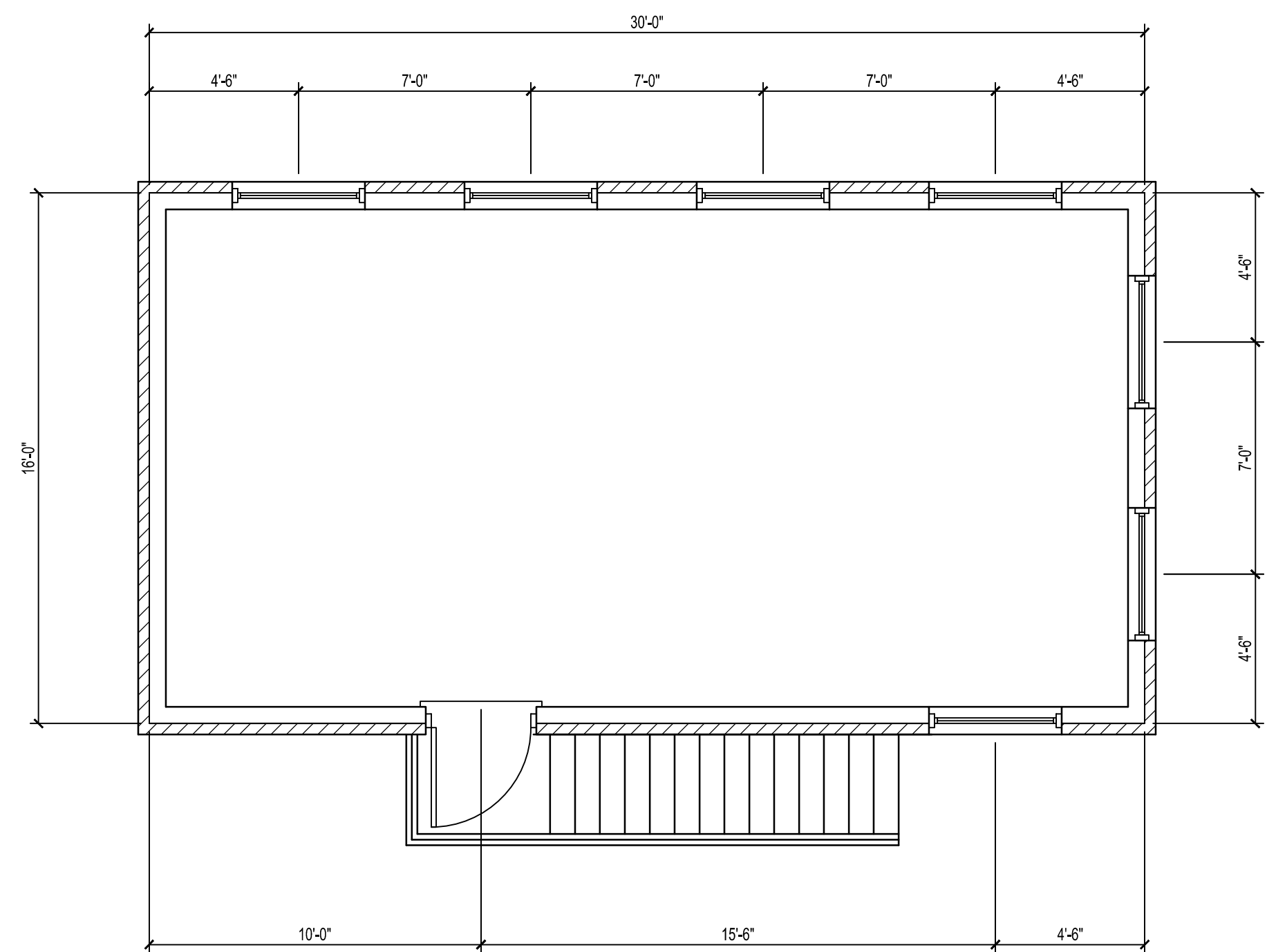
SECOND FLOOR PLAN SCALE: 1/4"=1'
